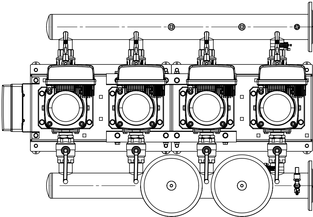
PLAN VIEW
