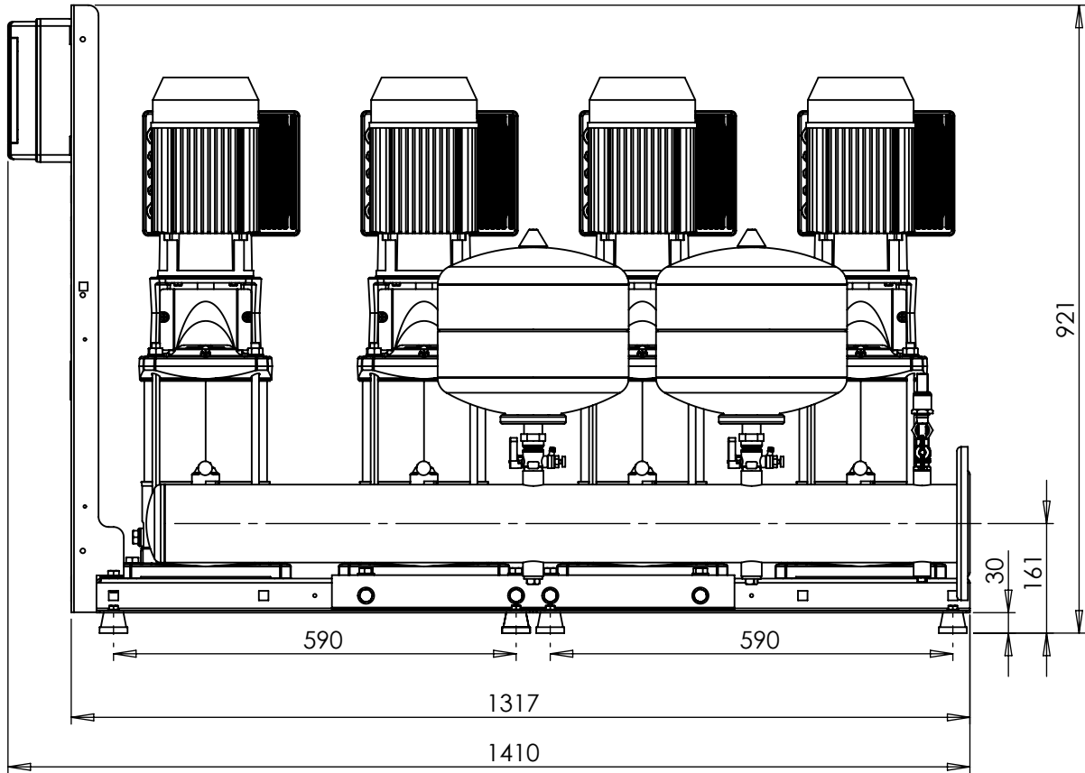
RIGHT VIEW
