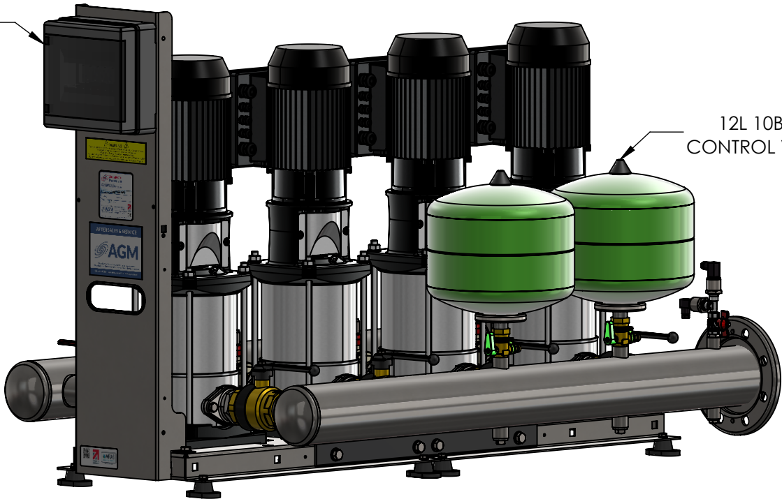
ISOMETRIC VIEW
