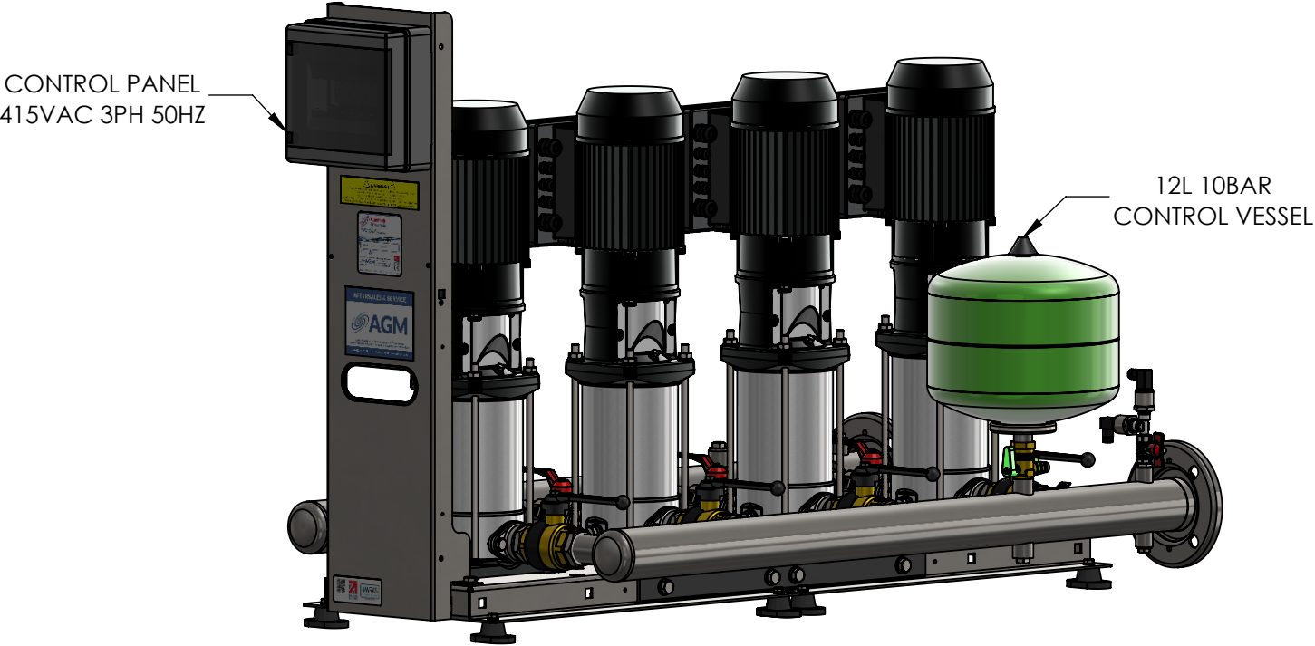
ISOMETRIC VIEW
