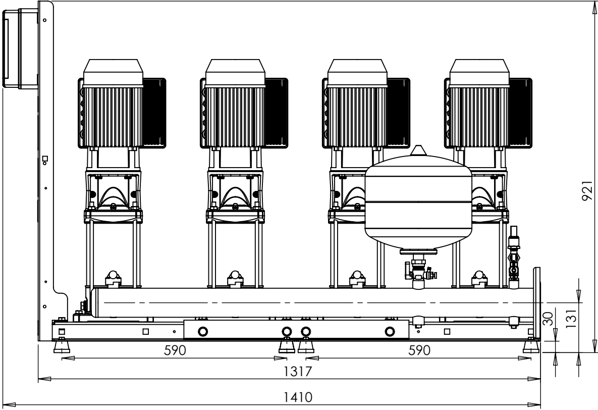
RIGHT VIEW
