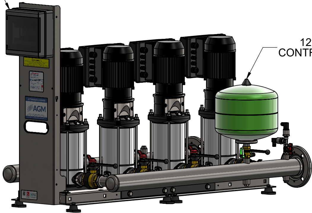
ISOMETRIC VIEW
