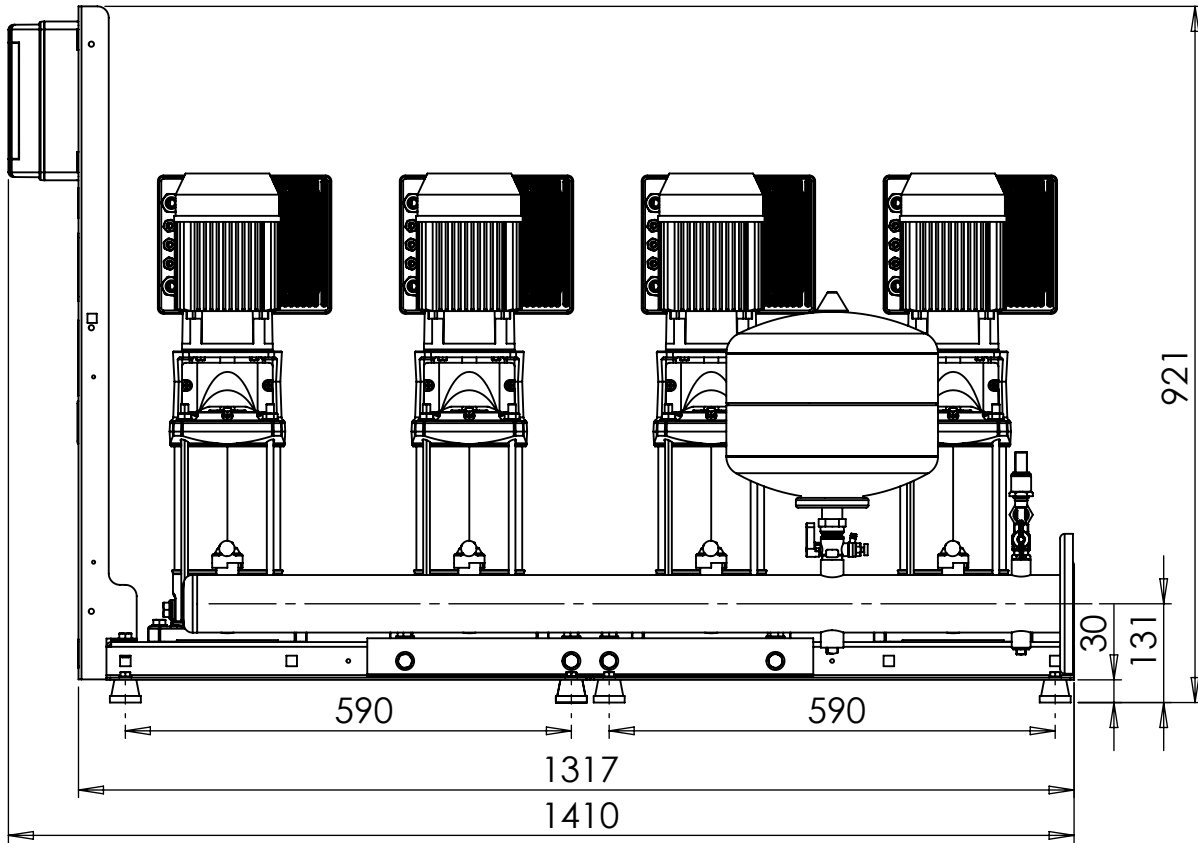
RIGHT VIEW
