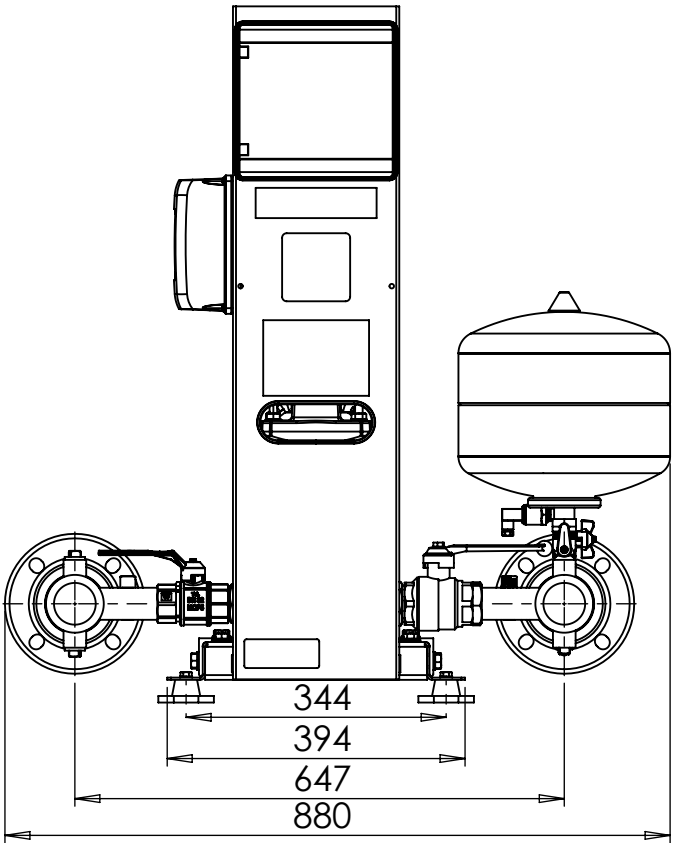
FRONT VIEW
