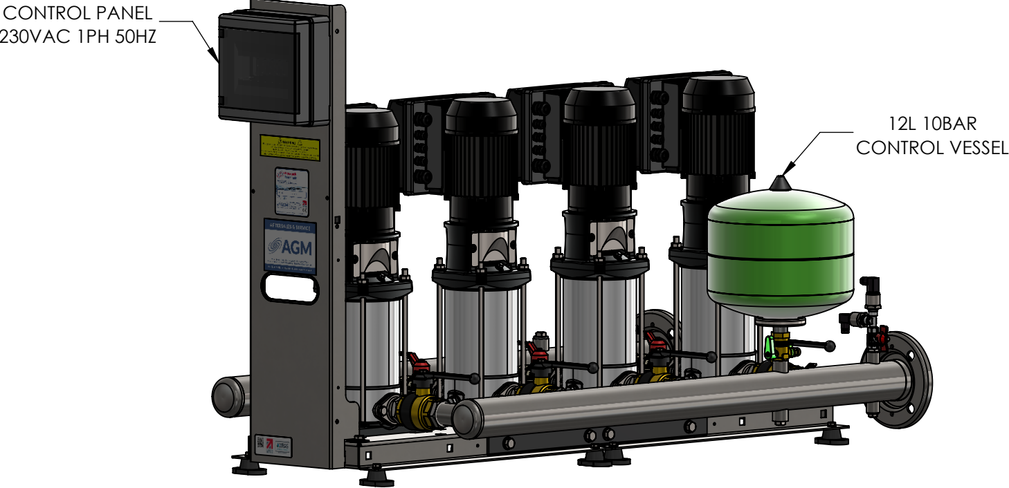
ISOMETRIC VIEW
