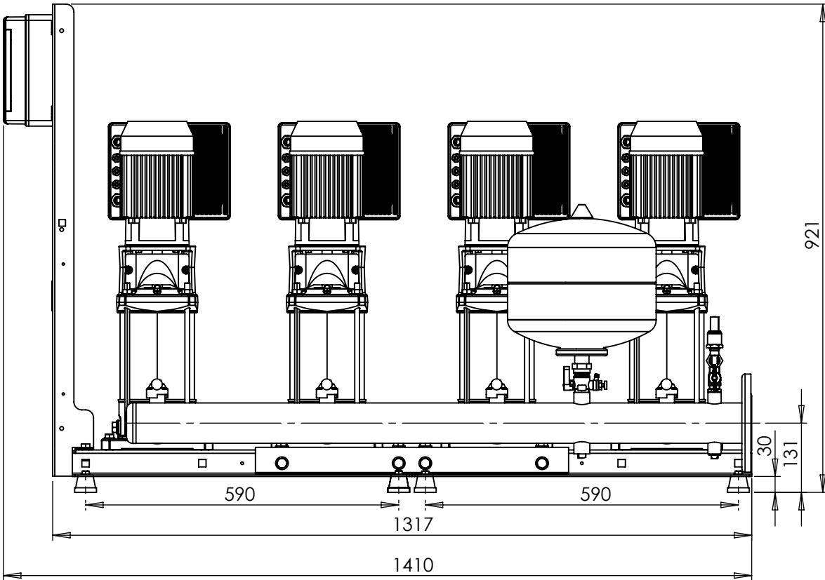
RIGHT VIEW
