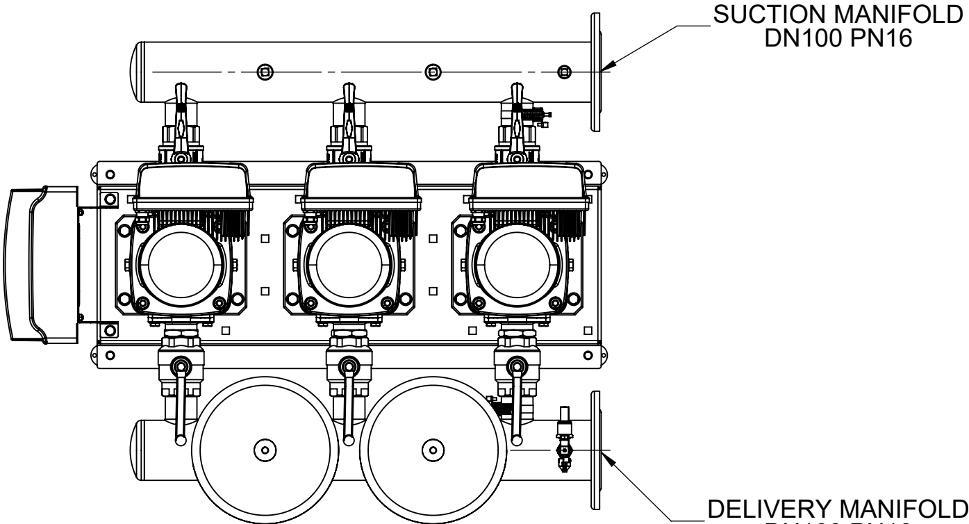
PLAN VIEW
