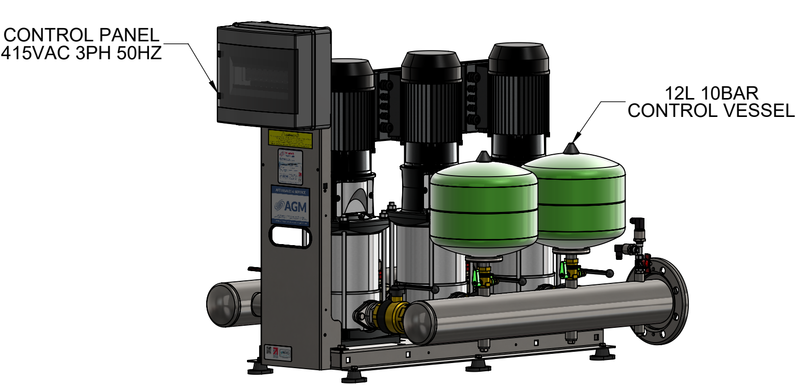
ISOMETRIC VIEW
