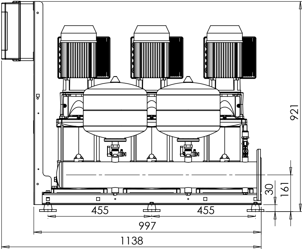
RIGHT VIEW
