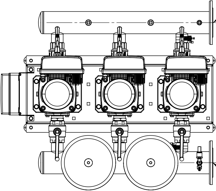
PLAN VIEW
