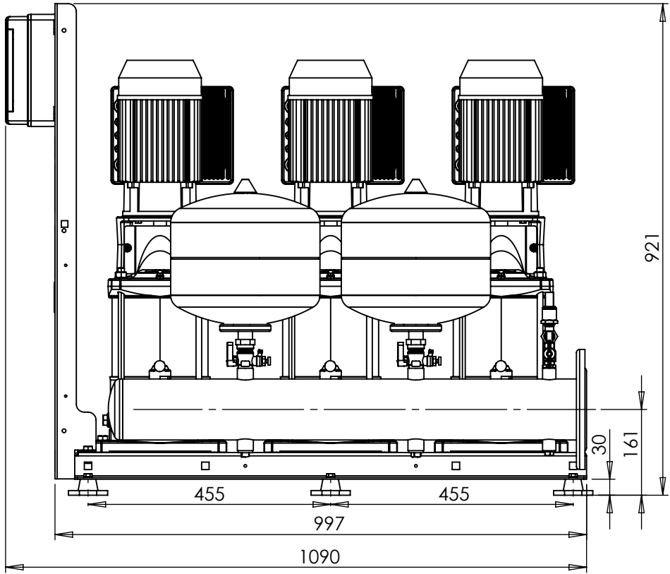
RIGHT VIEW
