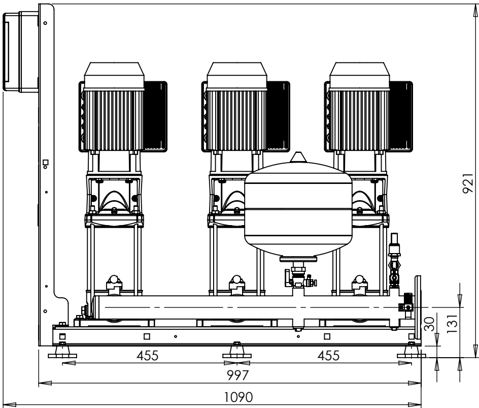
RIGHT VIEW
