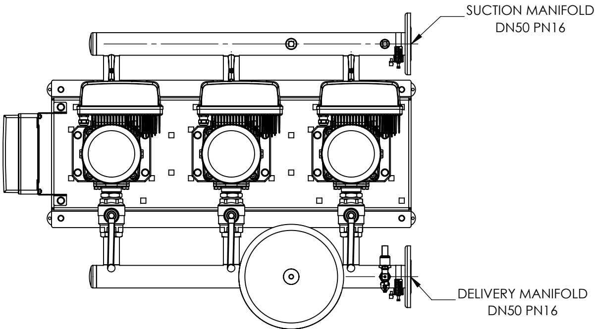
PLAN VIEW
