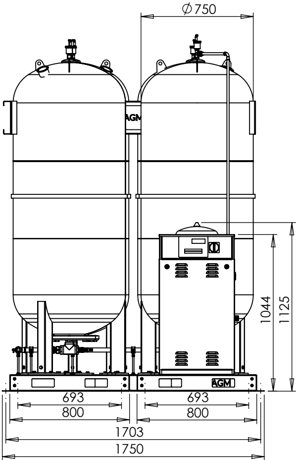
FRONT VIEW
