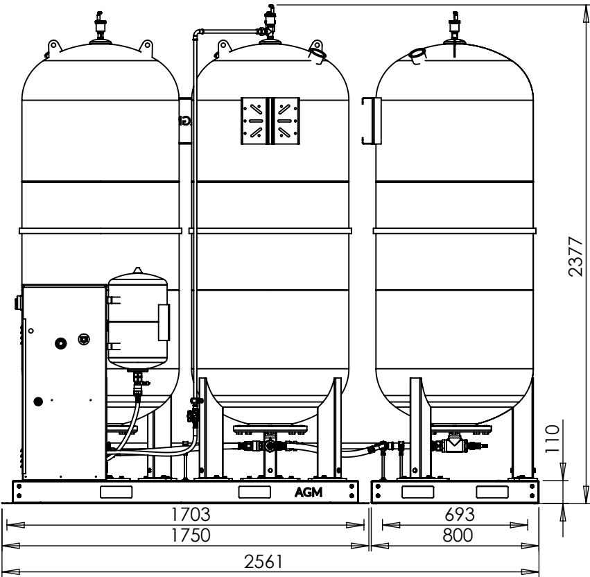
RIGHT VIEW
