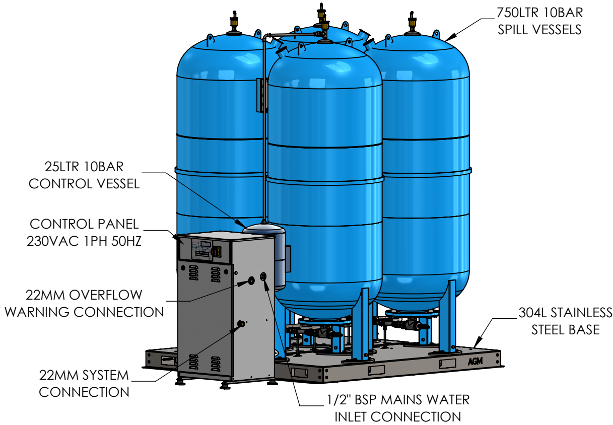
ISOMETRIC VIEW
