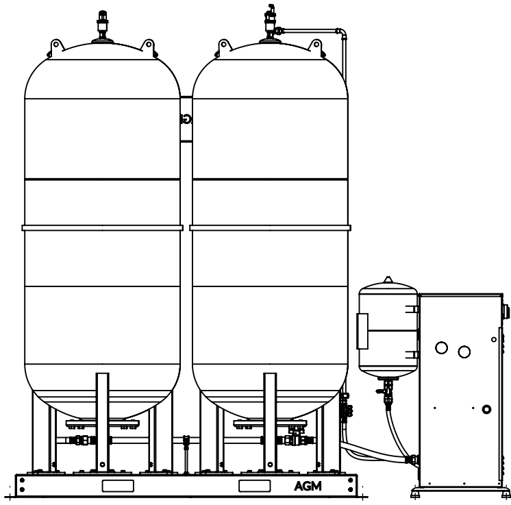
LEFT VIEW
