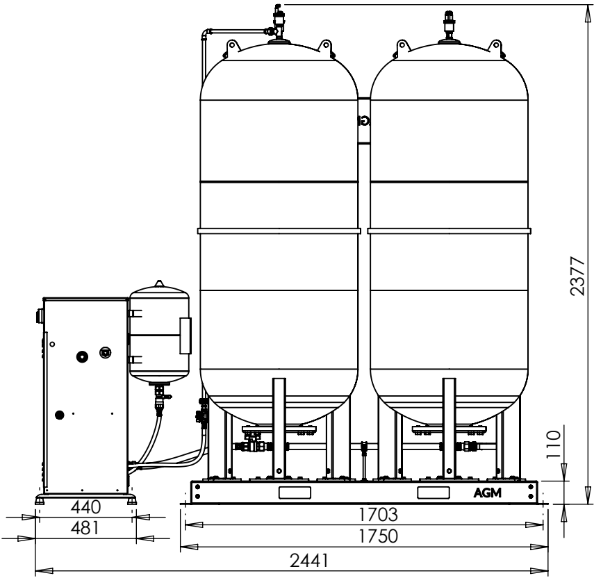
RIGHT VIEW
