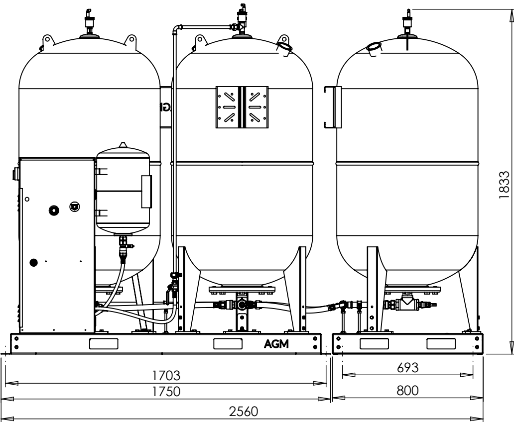
RIGHT VIEW
