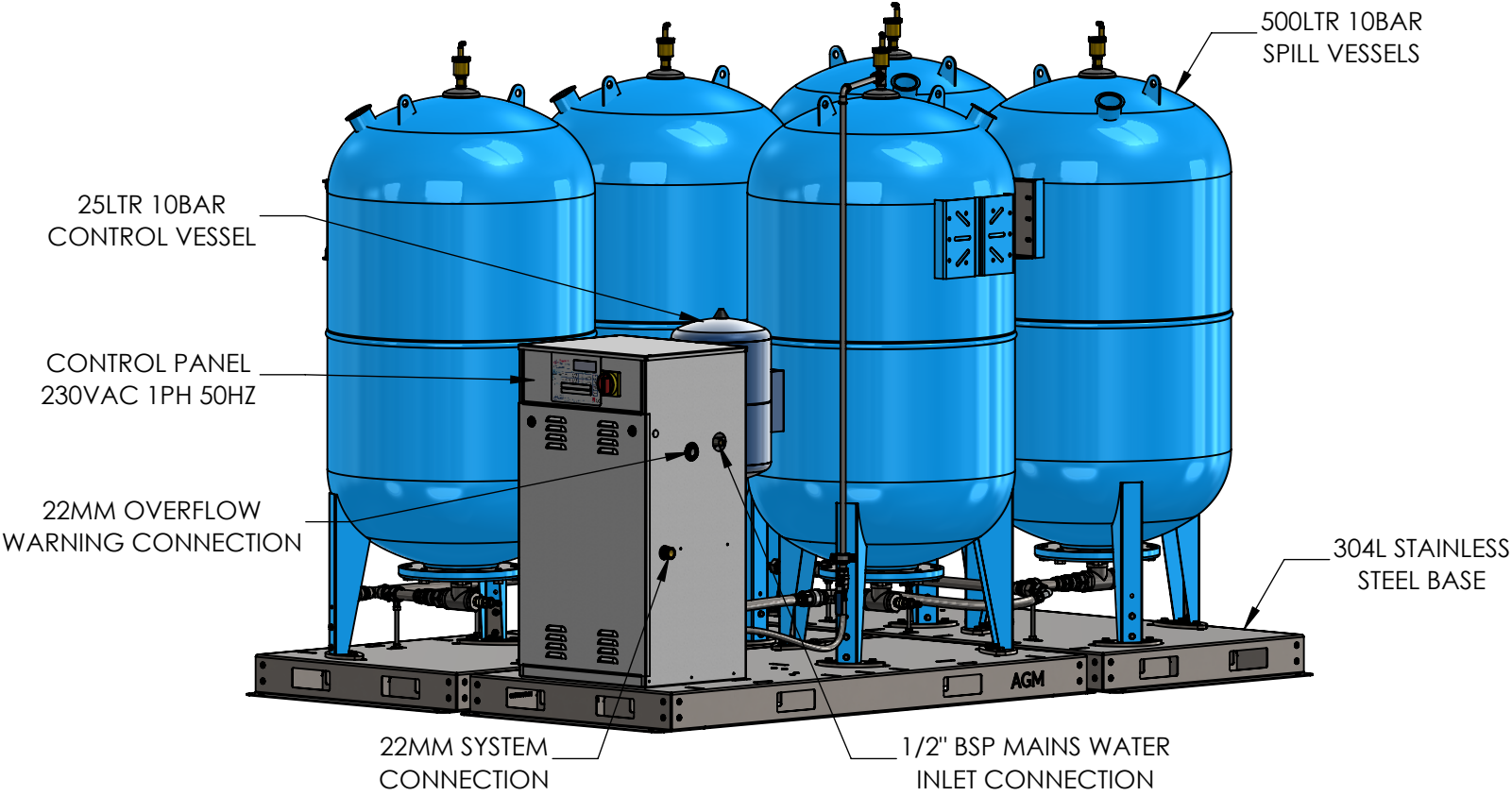
ISOMETRIC VIEW
