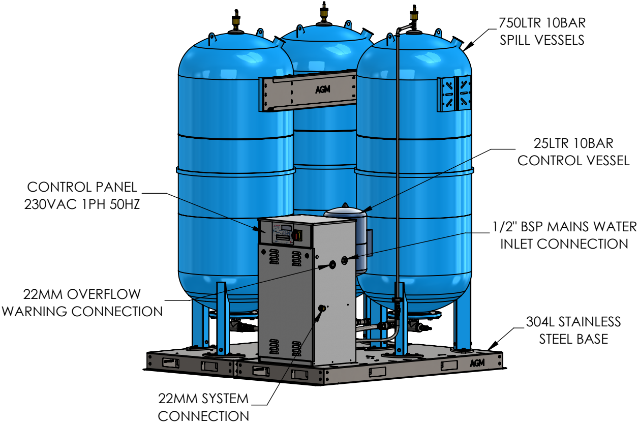
ISOMETRIC VIEW
