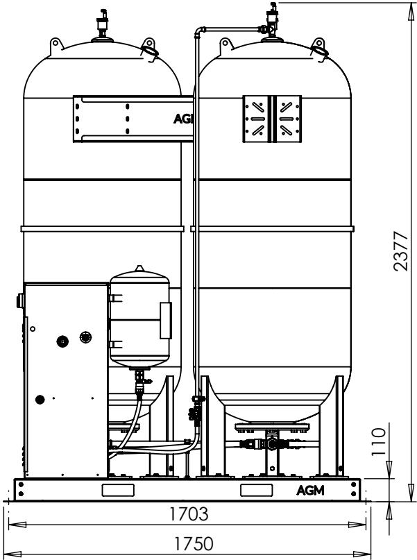
RIGHT VIEW
