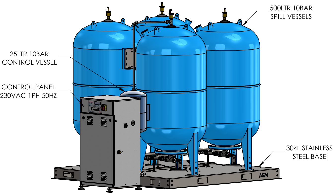
ISOMETRIC VIEW
