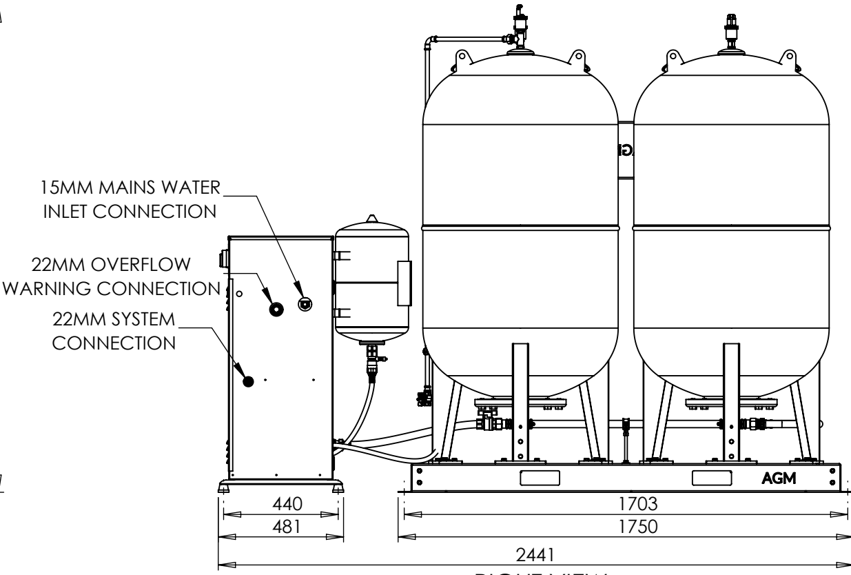
RIGHT VIEW
