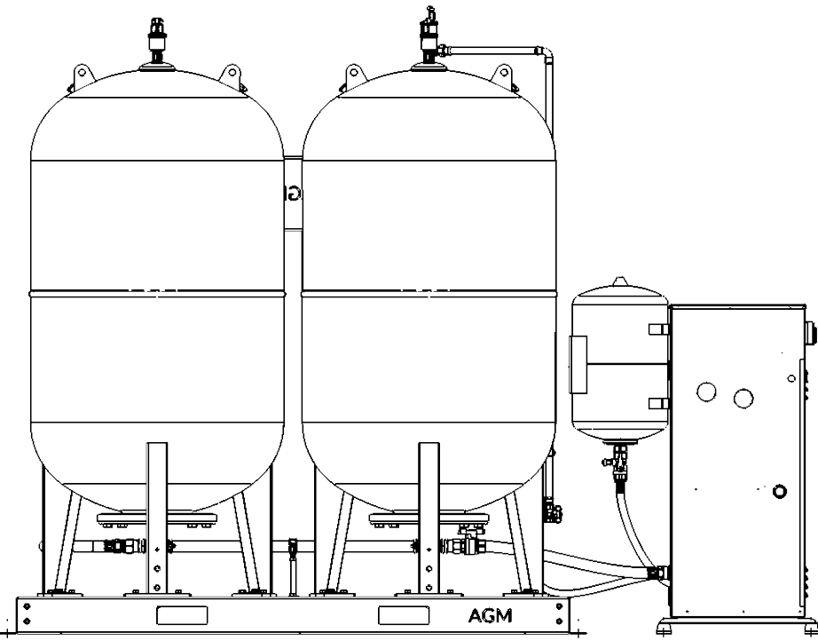
LEFT VIEW
