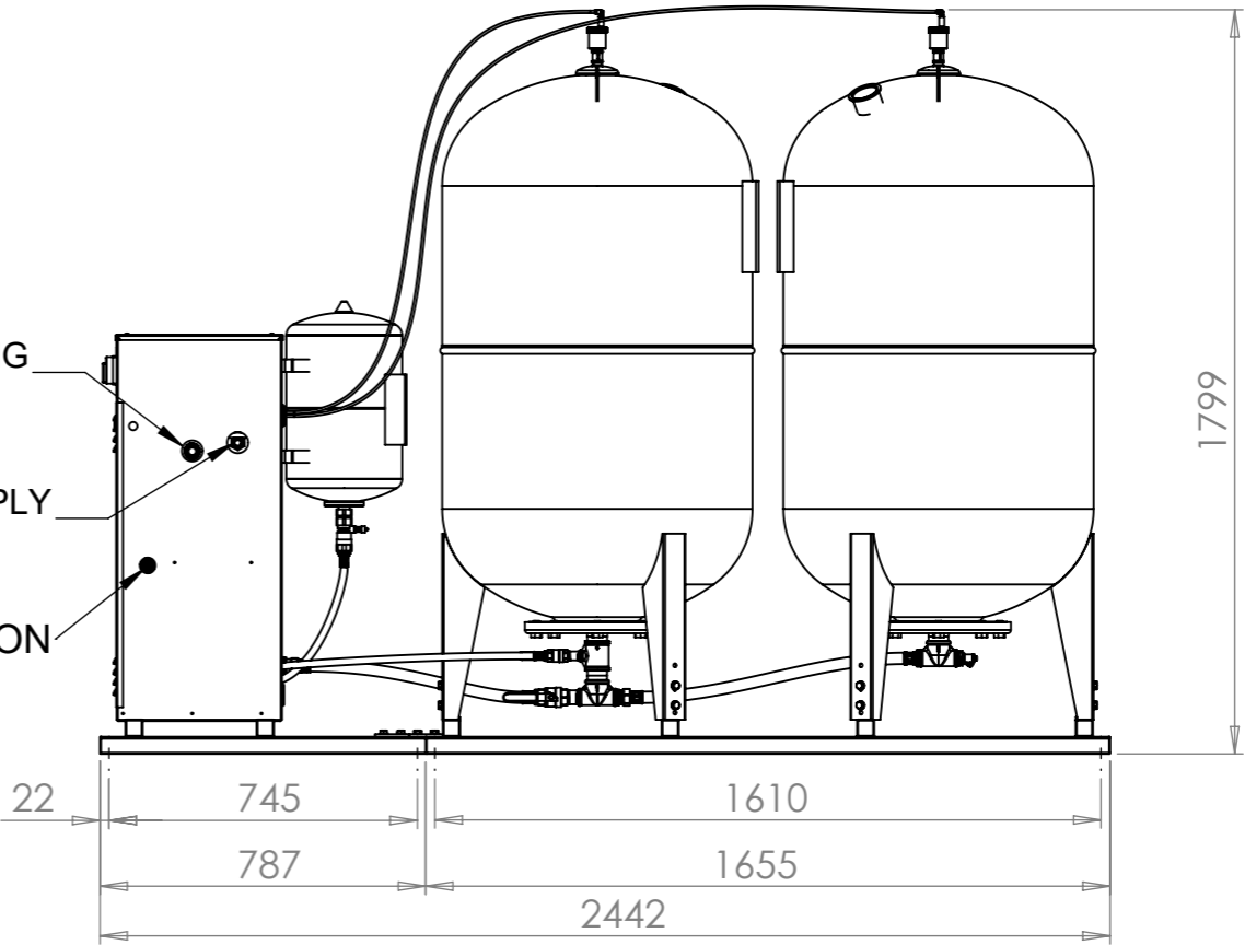
RIGHT VIEW
