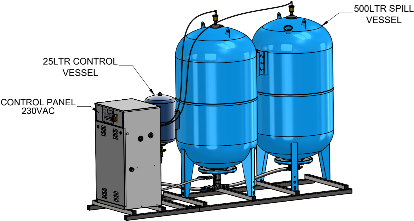
3D VIEW
