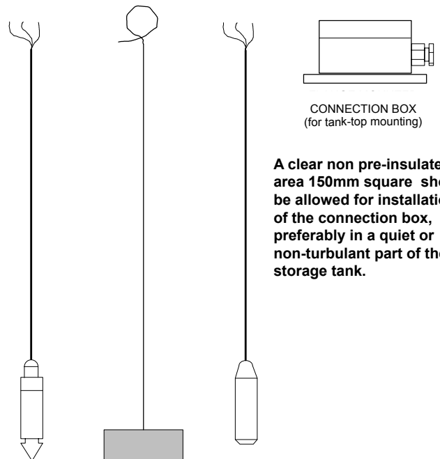
SUBMERGED LEVEL TRANSDUCER
